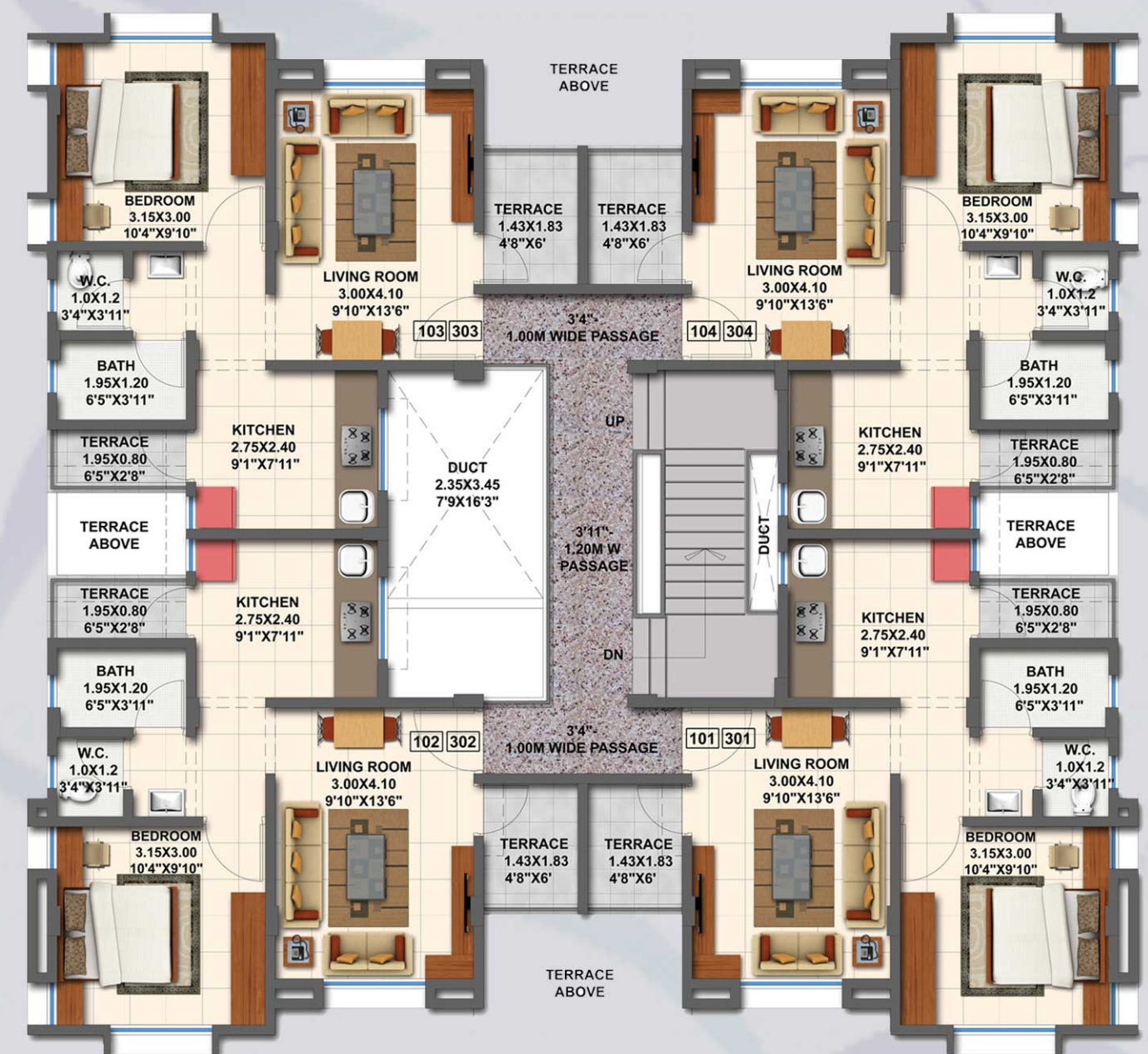
FIRST & THIRD FLOOR PLAN
